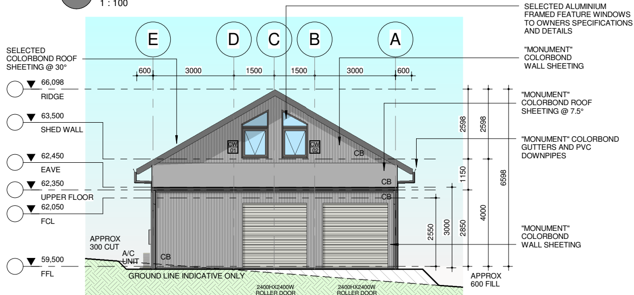
WESTERN ELEVATION 1 : 100
