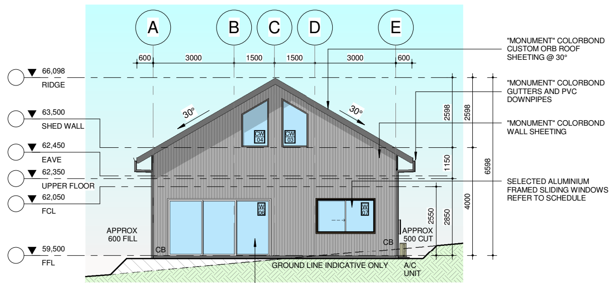
EASTERN ELEVATION 1 : 100
